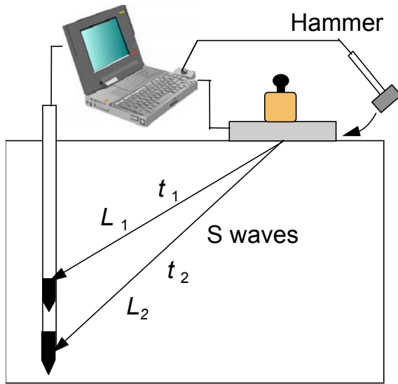
Figure 2 Seismic test
